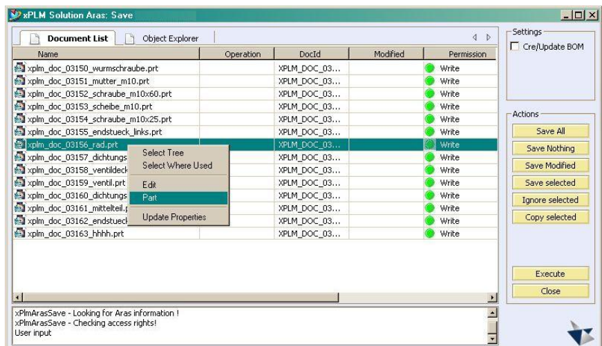
Save Dialog (List)
