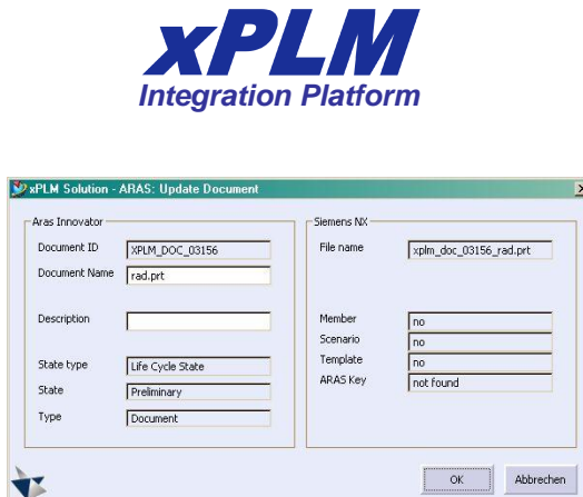
Save Dialog
